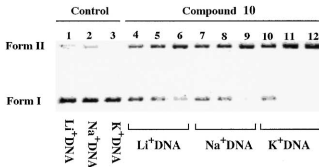
Figure 1. Cleavage of supercoiled (Form I) \text{Li}^+ -, \text{Na}^+ -, and \text{K}^+ -DNA by bis(propargylic) sulfone crown ether 10b . Solutions of pH 7.4 M + DNA (23 \mu\text{M} base pairs) containing 12.5% v/v DMSO were incubated for 18 h at 25°C with compound 10b . Samples were heated at 70°C for 90 s then mixed with loading buffer, and the nicked DNA products (form II) separated from supercoiled (form I) DNA by electrophoresis (0.7% agarose, TBE buffer, 45 V, 3 h) followed by ethidium bromide fluorescence imaging. Lane 1, \text{Li}^+ -DNA control; lane 2, \text{Na}^+ -DNA control; lane 3, \text{K}^+ -DNA control; lane 4, 10b (7.5 mM) + \text{Li}^+ -DNA; lane 5, 10b (10 mM) + \text{Li}^+ -DNA; lane 6, 10b (15 mM) + \text{Li}^+ -DNA; lane 7, 10b (7.5 mM) + \text{Na}^+ -DNA; lane 8, 10b (10 mM) + \text{Na}^+ -DNA; lane 9, 10b (15 mM) + \text{Na}^+ -DNA; lane 10, 10b (7.5 mM) + \text{K}^+ -DNA; lane 11, 10b (10 mM) + \text{K}^+ -DNA; lane 12, 10b (15 mM) + \text{K}^+ -DNA.
