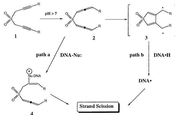
Scheme 1. DNA cleavage by bis(propargylic) sulfones.
