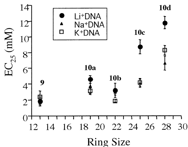
Figure 2. DNA cleavage efficiency, expressed as \text{EC}_{25} , the concentration of compound required to effect 25% normalized cleavage of supercoiled DNA, as a function of ring size and alkali metal ion for bis(propargylic) sulfones 9 and 10a–d .
