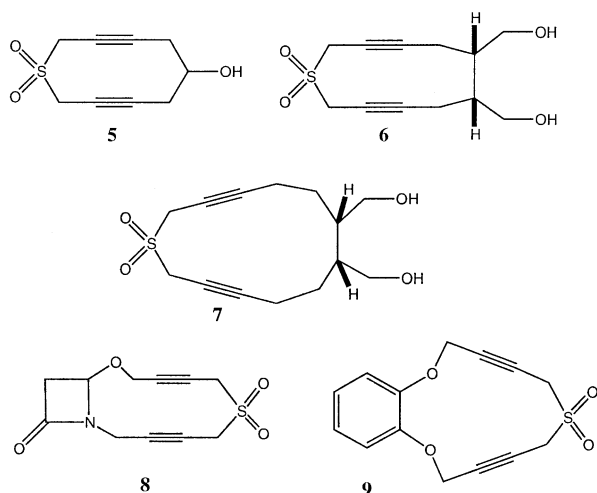
Scheme 2. Structures of cyclic bis(propargylic) sulfones.
