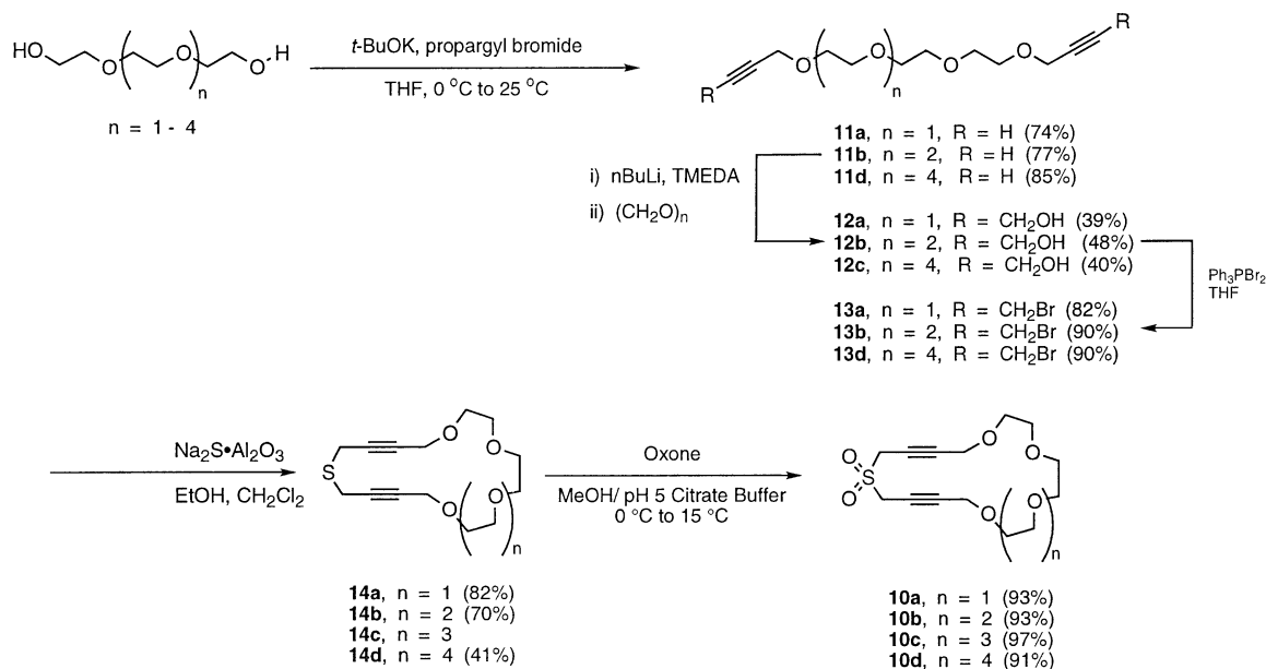
Scheme 3. Synthesis of crown ethers.
